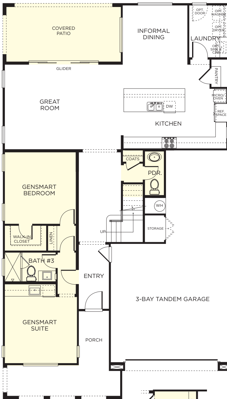
FIRST FLOOR
