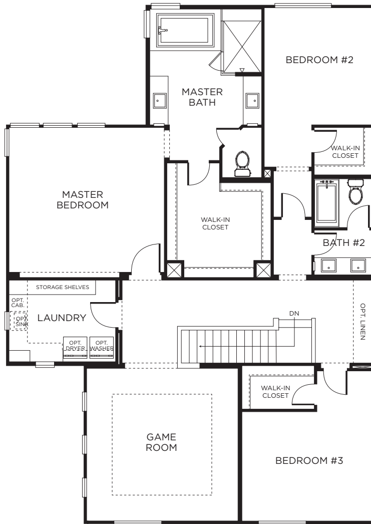
SECOND FLOOR
